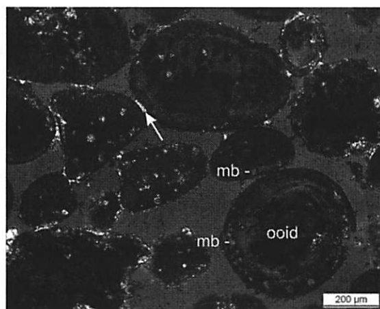
Figure 3. Sample CCI, core # 12, 2.0 mbs. Microfacies of Unit 1 : poorly cemented oolitic-peloidal grainstone. Note rare low-Mg calcite meniscus cement (white arrow), partial micritization of ooids, and numerous microborings (mb) of probable algal origin.
